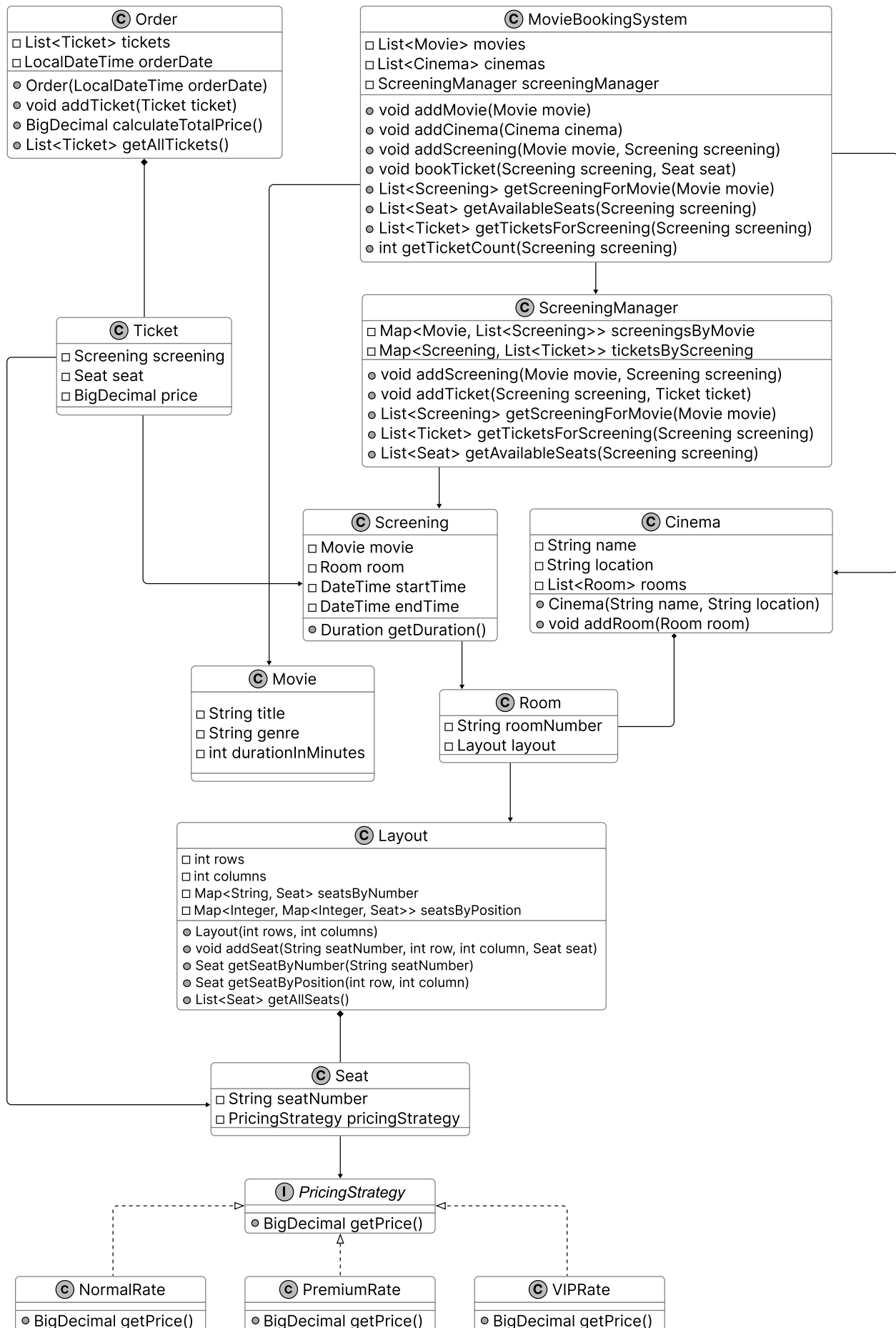
Class Diagram of Movie Ticket Booking System
